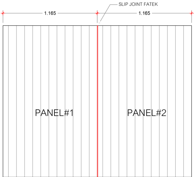
DETAIL JOINT OF PANEL
