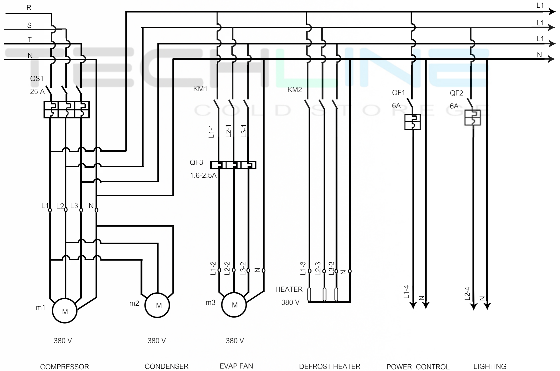
DIAGRAM CONTROLER COLD ROOM
